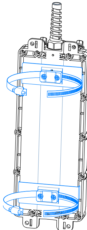
POLE MOUNT KIT
